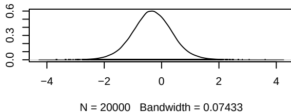
Density of d.Osimertinib.Gefitinib_Erlotinib
