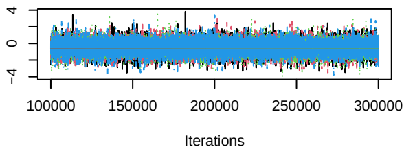
Trace of d.Afatinib.Afatinib_Cetuximab
