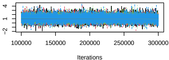
Trace of d.Afatinib.chemo
