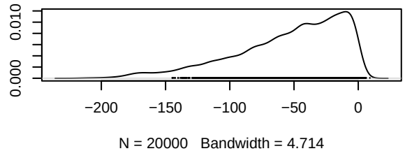
Density of d.Osimertinib.Osimertinib_PD_L1i
