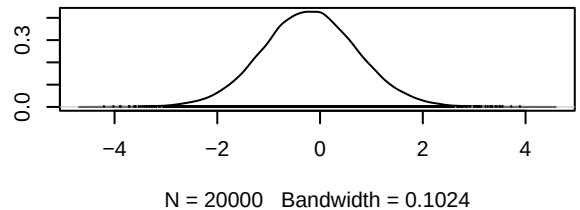
Density of d.Placebo.Afatinib
