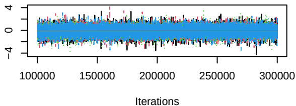
Trace of d.Gefitinib.Dacomitinib
