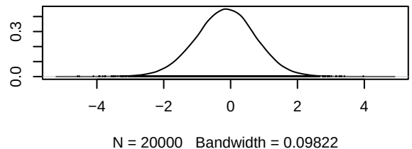
Density of d.Placebo.Gefitinib
