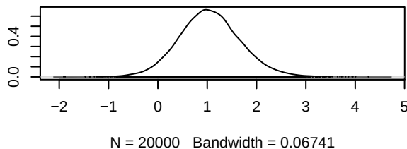
Density of d.Afatinib.chemo
