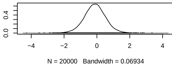
Density of d.Gefitinib.Dacomitinib
